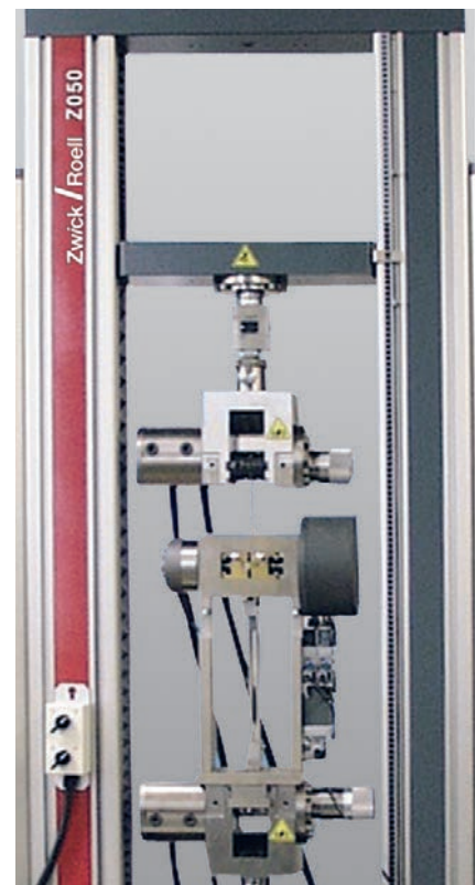
Fig.3: Z050 materials testing machine with draw-bead tool
