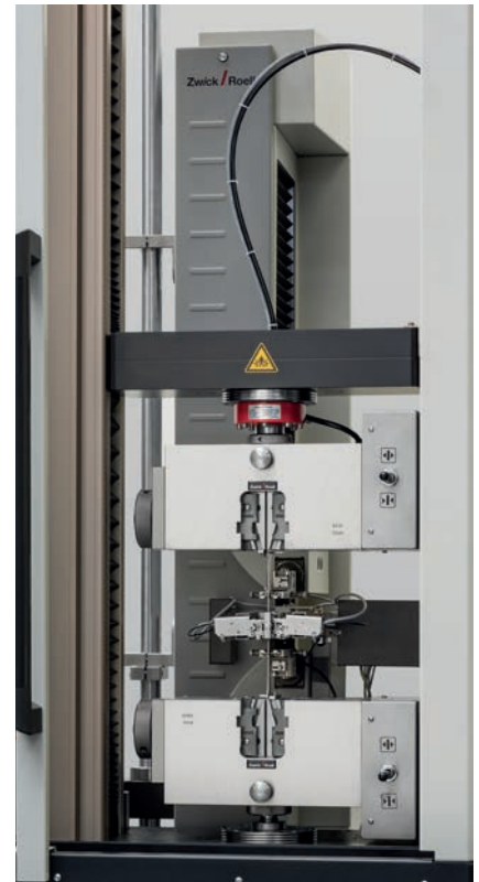
Fig. 4: multiXtens with optional fine-strain and transverse-strain measurement
