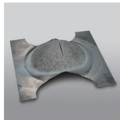
Fig.4: Specimen from FLC test (Nakajima)
