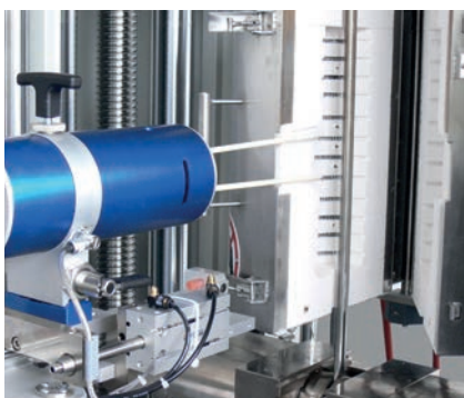
Fig.2: High-temperature furnace with HT extensometer
