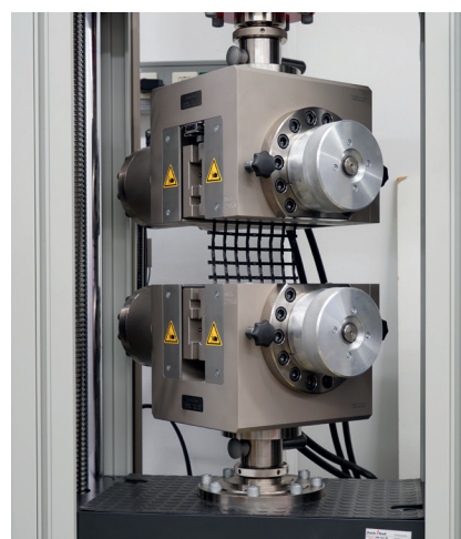
Fig. 5. Hydraulic grips for geotextiles
