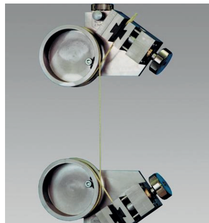
Fig. 4. Rope grips
