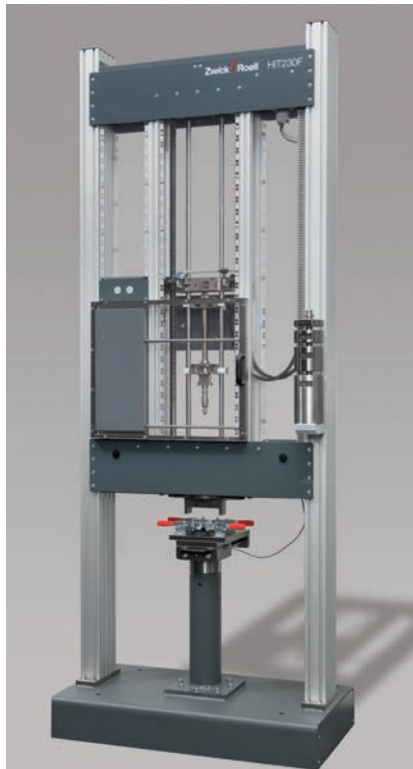
Fig. 1: HIT 230F drop weight tester with accessories for CAI pre-damaging
