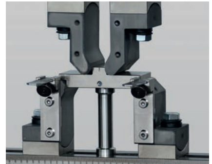
Fig. 5: Adjustment gauge for the 4-point flexure test arrangement
