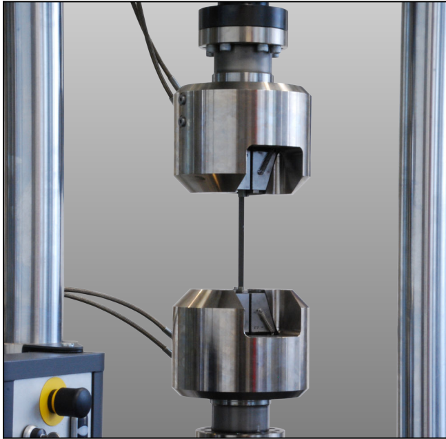
BOW-100 hydraulic wedge grips
