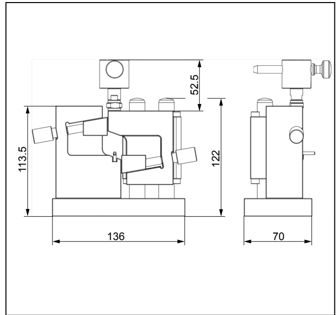
Shear test device dimensions
