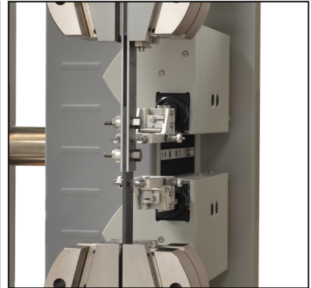
Bearing-strength test fixture as per ASTM D7248 Method A
