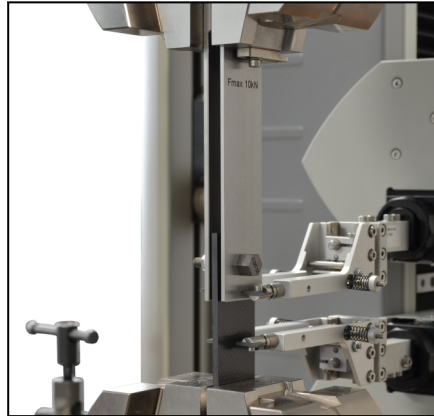
Bearing-strength test fixture as per ASTM D5961 Method A / ISO 12815
