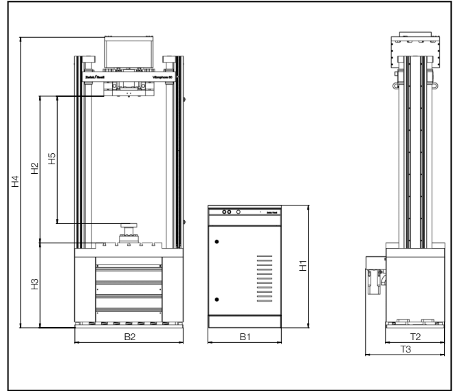
Drawing: Vibrophore 50
