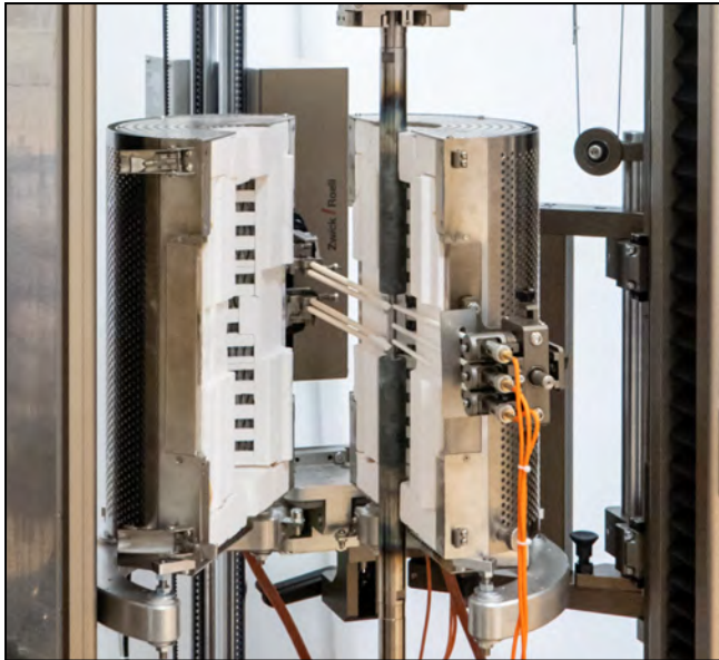
makroXtens II 100 HP on high-temperature furnace HTF-LVW 1,250 °C
